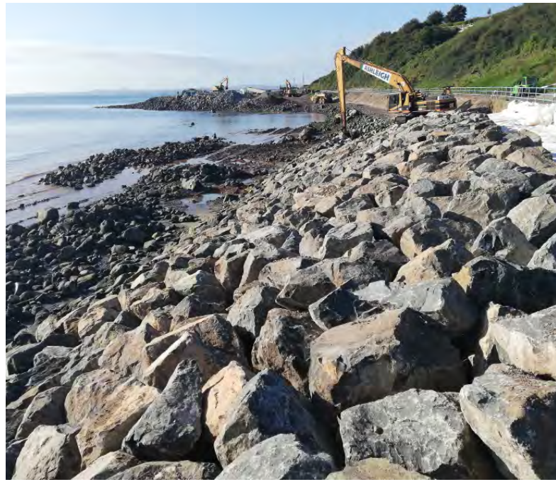
Rock armour revetment
