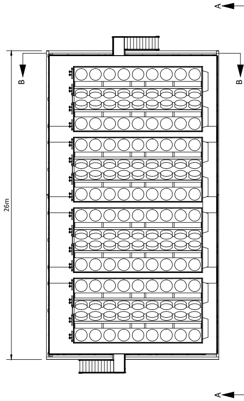
PLAN VIEW
